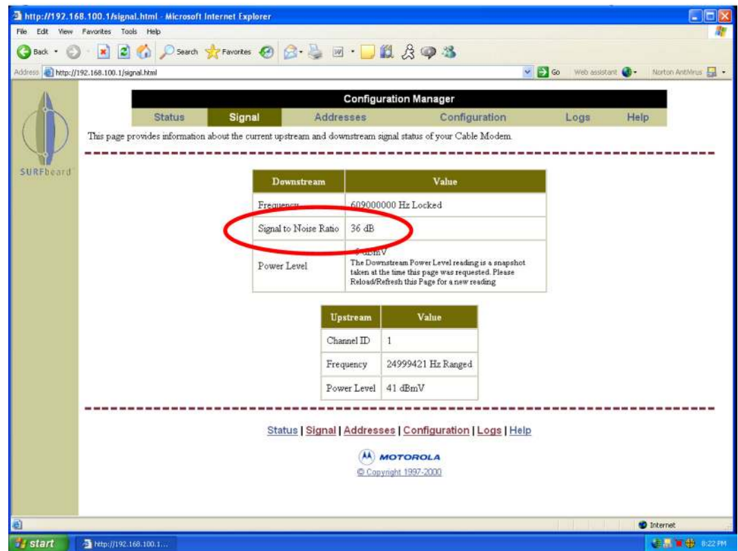
Figure 10. Cable Modem Diagnostics Screen Showing Downstream Equalized SNR (RxMER)
