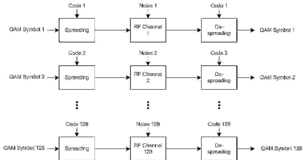
Figure 22. Conceptually, S-CDMA Can Be Thought of as Having an Independent Upstream Channel for Each Code, Each with Its Own Noise Component.
