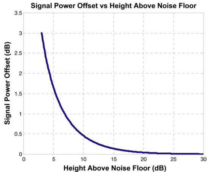
Figure 8. Signal Power Measurement Correction Relative to Noise Floor
