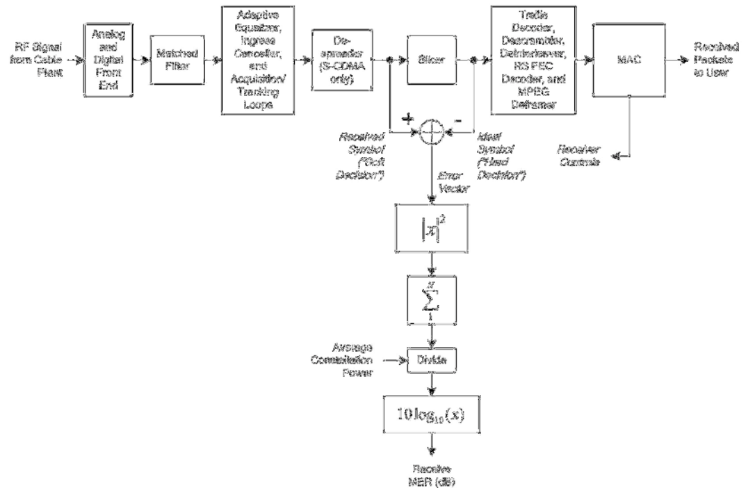
Figure 11. Block Diagram of Generalized Digital QAM Receiver, Showing Computation of Receive MER
