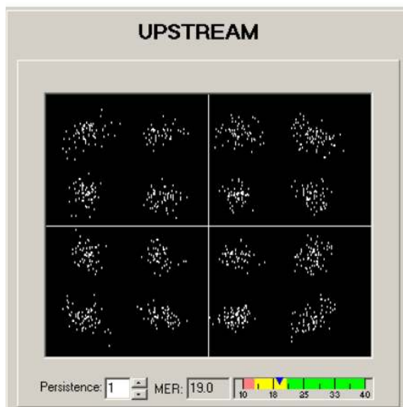
Figure 18. Impaired 16-QAM Digitally Modulated Signal; the Unequalized MER Is 19 dB (Courtesy Filtronic-Sigtek)
