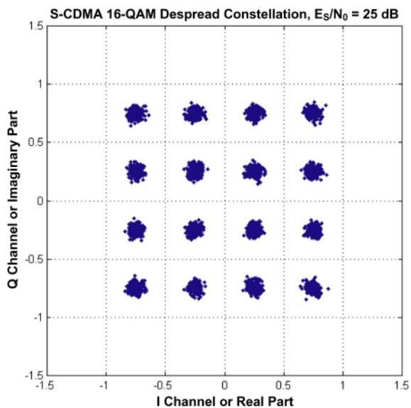
Figure 23. S-CDMA 16-QAM Constellation with 25-dB RxMER
