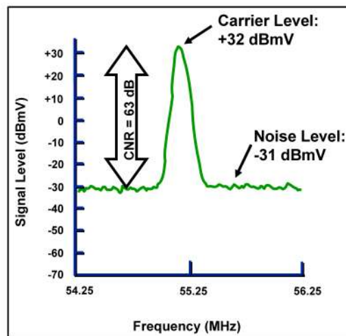
Figure 1. RF CNR Measurement (as detected in the test equipment resolution bandwidth)
