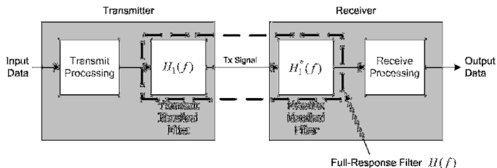
Figure 3. General Digital Communications System Showing Matched Filters in Transmitter and Receiver
