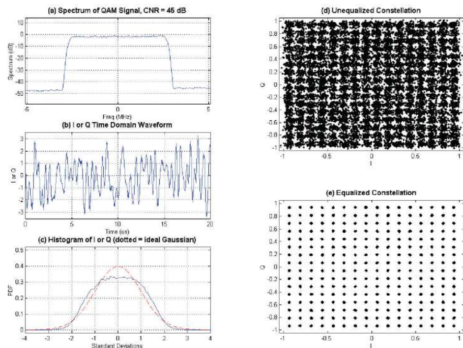
(a) Spectrum Display (b) Time Domain Showing I or Q Baseband Waveform (c) Histogram of I or Q Baseband Signal, Approximating Gaussian Distribution (d) Received Constellation Before Channel Response Is Equalized; RxMER = 26 dB (e) Received Constellation After Equalization; RxMER = 45 dB
