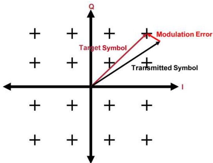
Figure 13. Modulation Error Is a Measure of Modulation Quality. (Source: Hewlett-Packard)
