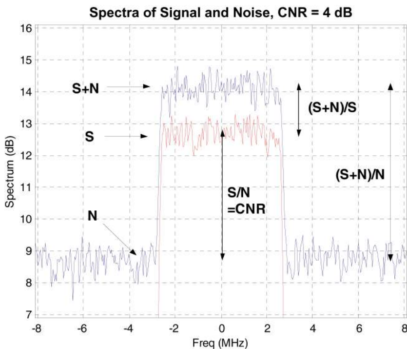
Figure 7. Close-Up View of Signal and Noise as Measured on a Spectrum Analyzer
