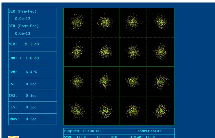
Figure 20. Upstream Unequalized MER for the Digitally Modulated Signal in Figure 19 Is Only 21 dB, and the EVM Is a Relatively High 6.4 Percent. (Courtesy Sunrise Telecom)
