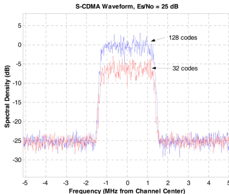
Figure 24. S-CDMA Upstream Spectrum with E_s/N_0 per Code = 25 dB.
