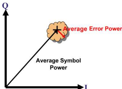
Figure 14. Modulation Error Ratio Is the Ratio of Average Symbol Power to Average Error Power. (Source: Hewlett-Packard)
