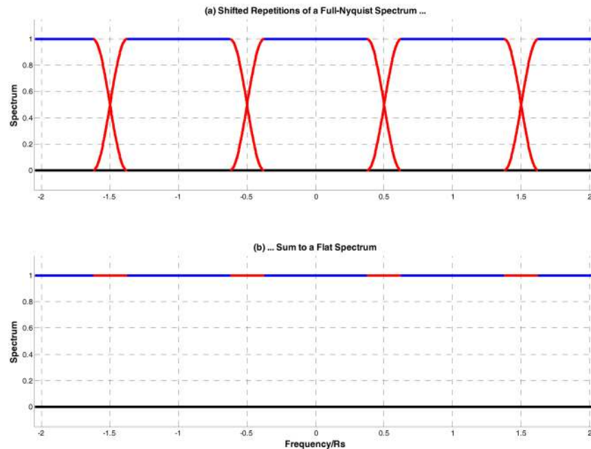
Figure 5. The Nyquist Property States that When Copies of the Spectrum Are Shifted by Multiples of the Symbol Rate and Added, the Result Is a Flat Spectrum, Which Results in Zero ISI.
