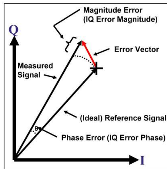
Figure 12. The Error Vector Is the Difference Between the Measured Signal (Soft Decision) and the Reference or Target Signal (Hard Decision). (Source: Hewlett-Packard)
