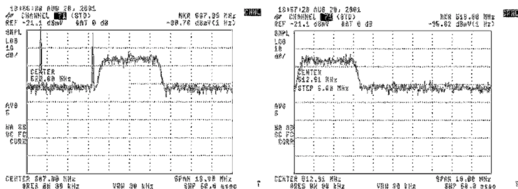
Figure 6. Digitally Modulated Signal CNR (This Example Shows an Approximate CNR of 15 dB.)
