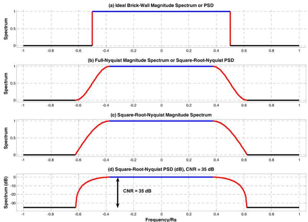
Figure 4. Ideal QAM Spectrum Plots
